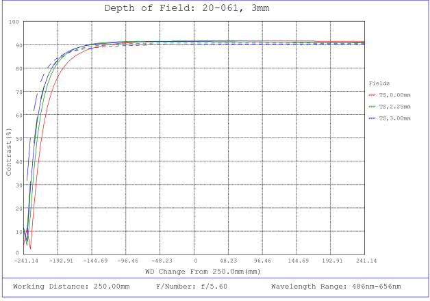
#20-061, 3mm FL f/5.6 IR-Cut Rugged Blue Series M12 Lens, Depth of Field Plot, 250mm Working Distance, f5.6
