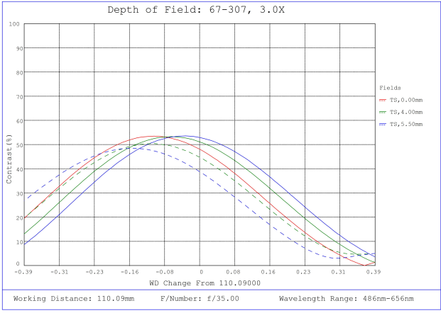
#67-307, 3X, 110mm WD, In-Line CompactTL™ Telecentric Lens, Depth of Field Plot, 110mm Working Distance, f35
