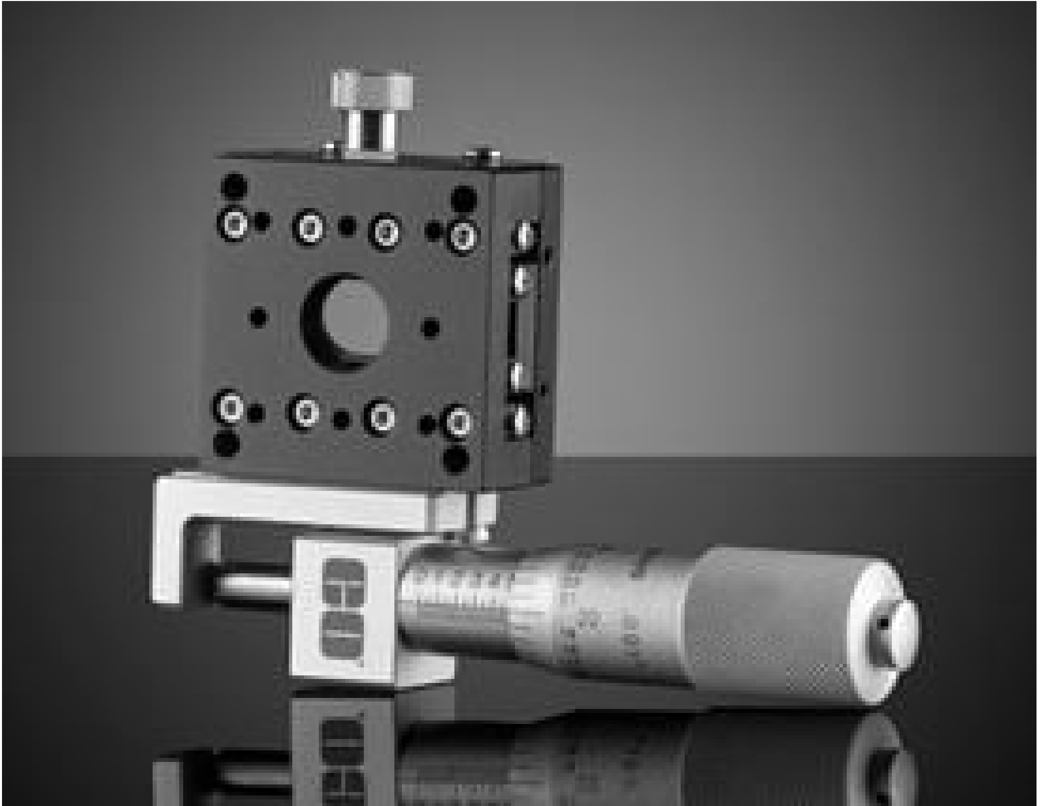
40mm, Side Drive, Thru-Hole Micrometer Stage
