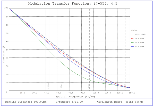
#87-556, 4.5mm, f/11 Ci Series Fixed Focal Length Lens, Modulated Transfer Function (MTF) Plot, 500mm Working Distance, f11
