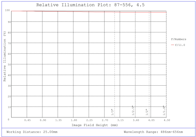
#87-556, 4.5mm, f/11 Ci Series Fixed Focal Length Lens, Relative Illumination Plot
