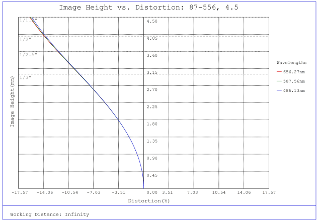
#87-556, 4.5mm, f/11 Ci Series Fixed Focal Length Lens, Distortion Plot
