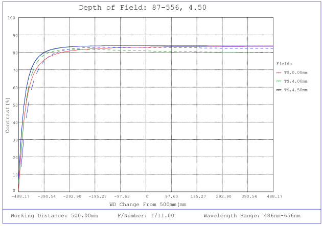
#87-556, 4.5mm, f/11 Ci Series Fixed Focal Length Lens, Depth of Field Plot, 500mm Working Distance, f11
