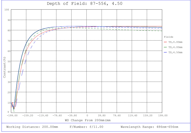
#87-556, 4.5mm, f/11 Ci Series Fixed Focal Length Lens, Depth of Field Plot, 200mm Working Distance, f11
