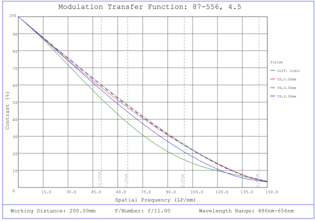
#87-556, 4.5mm, f/11 Ci Series Fixed Focal Length Lens, Modulated Transfer Function (MTF) Plot, 200mm Working Distance, f11
