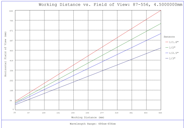
#87-556, 4.5mm, f/11 Ci Series Fixed Focal Length Lens, Working Distance versus Field of View Plot
