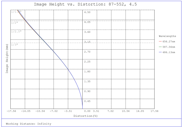
#87-552, 4.5mm, f/2.8 Ci Series Fixed Focal Length Lens, Distortion Plot
