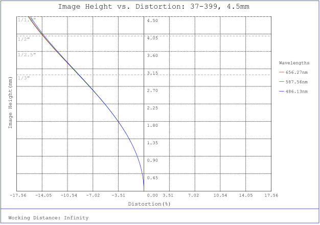
#37-399, 4.5mm, f/2.8 Cr Series Fixed Focal Length Lens, Distortion Plot
