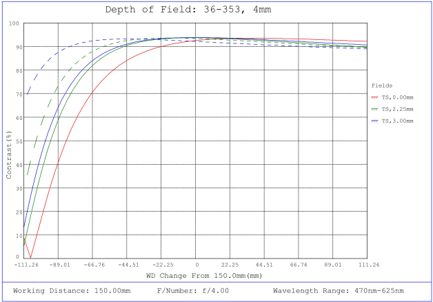
#36-353, 4mm FL f/4, Rugged Blue Series M12 Lens, Depth of Field Plot, 150mm Working Distance, f4
