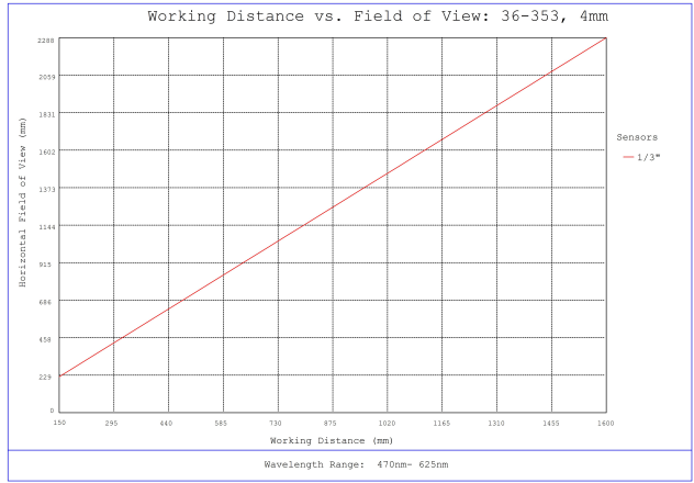
#36-353, 4mm FL f/4, Rugged Blue Series M12 Lens, Working Distance versus Field of View Plot
