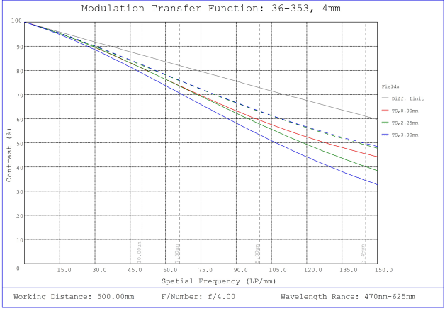
#36-353, 4mm FL f/4, Rugged Blue Series M12 Lens, Modulated Transfer Function (MTF) Plot, 500mm Working Distance, f4
