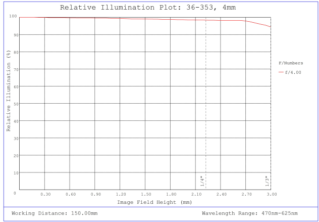
#36-353, 4mm FL f/4, Rugged Blue Series M12 Lens, Relative Illumination Plot
