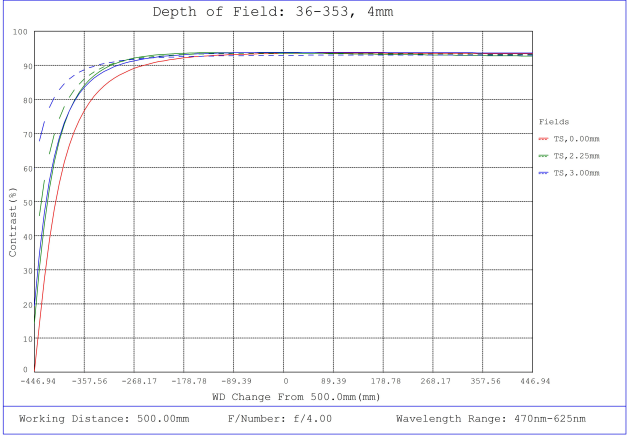
#36-353, 4mm FL f/4, Rugged Blue Series M12 Lens, Depth of Field Plot, 500mm Working Distance, f4
