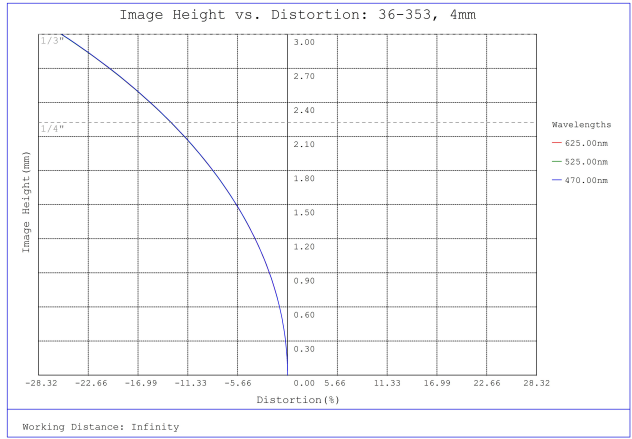
#36-353, 4mm FL f/4, Rugged Blue Series M12 Lens, Distortion Plot
