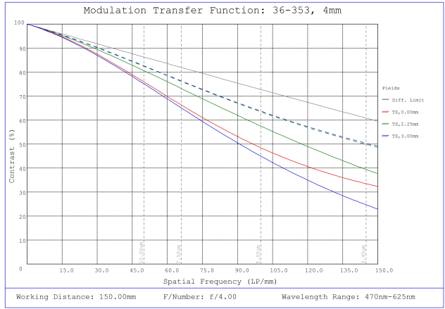
#36-353, 4mm FL f/4, Rugged Blue Series M12 Lens, Modulated Transfer Function (MTF) Plot, 150mm Working Distance, f4
