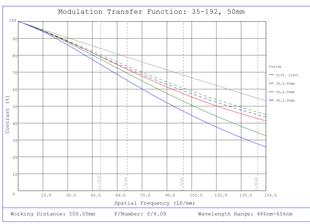
#35-192, 50mm, f/4.0 Cr Series Fixed Focal Length Lens, Modulated Transfer Function (MTF) Plot, 500mm Working Distance, f4
