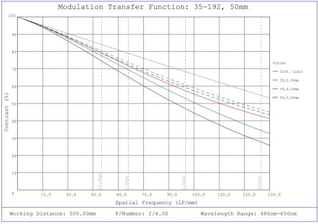
#35-192, 50mm, f/4.0 Cr Series Fixed Focal Length Lens, Modulated Transfer Function (MTF) Plot, 500mm Working Distance, f4
