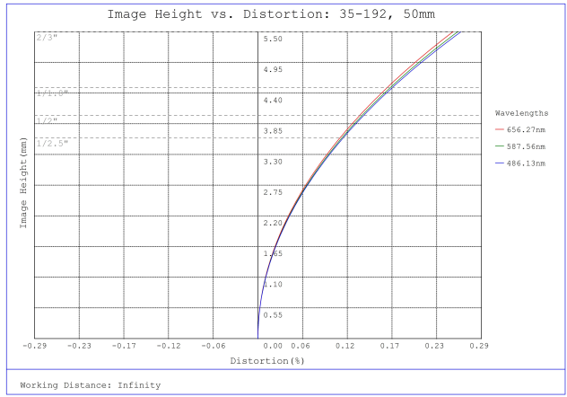
#35-192, 50mm, f/4.0 Cr Series Fixed Focal Length Lens, Distortion Plot
