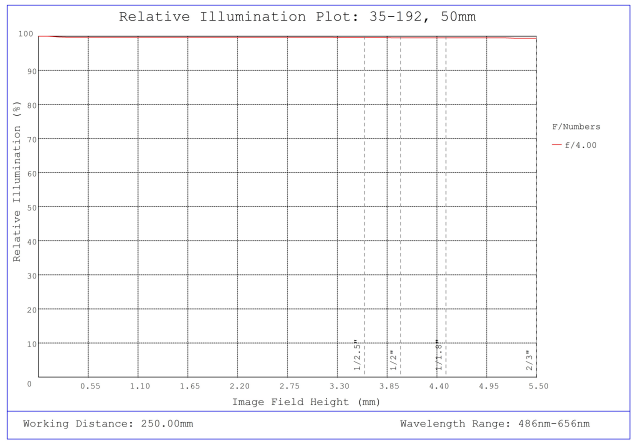
#35-192, 50mm, f/4.0 Cr Series Fixed Focal Length Lens, Relative Illumination Plot
