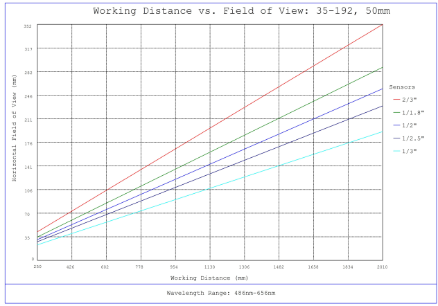
#35-192, 50mm, f/4.0 Cr Series Fixed Focal Length Lens, Working Distance versus Field of View Plot
