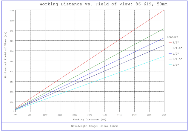
#86-619, 50mm, f/11.0 Ci Series Fixed Focal Length Lens, Working Distance versus Field of View Plot
