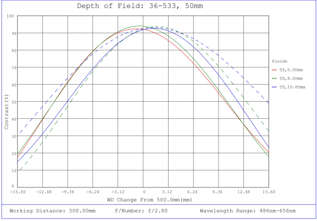
#36-533, 50mm f/2.8, HPr Series Fixed Focal Length Lens, Depth of Field Plot, 500mm Working Distance, f2.8
