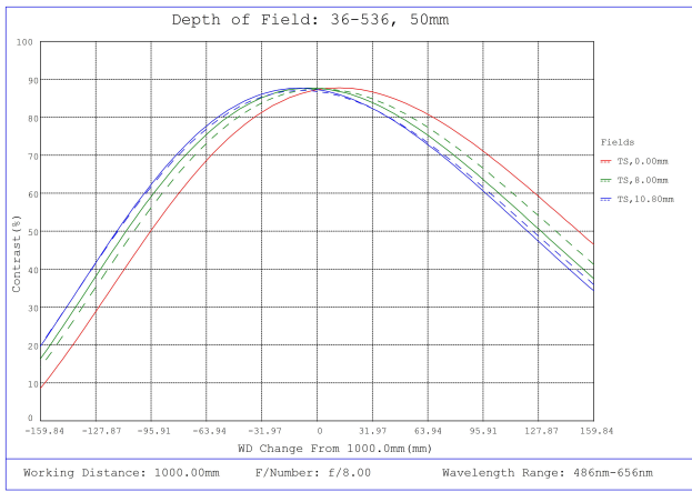
#36-536, 50mm f/8.0, HPr Series Fixed Focal Length Lens, Depth of Field Plot, 1000mm Working Distance, f8
