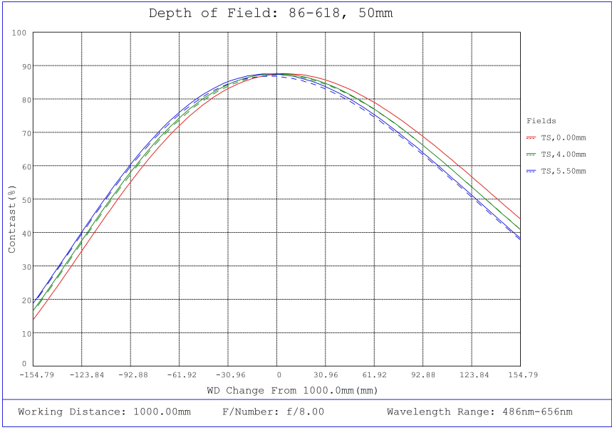
#86-618, 50mm, f/8.0 Ci Series Fixed Focal Length Lens, Depth of Field Plot, 1000mm Working Distance, f8
