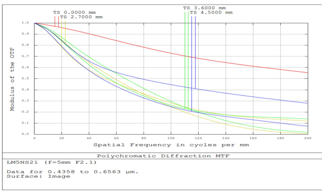
5mm FL, f/2.1, Low Distortion M12 Lens, MTF Plot
