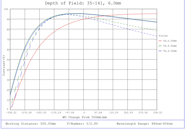
#35-141, 6mm, f/2.8 Cr Series Fixed Focal Length Lens, Depth of Field Plot, 500mm Working Distance, f2.8
