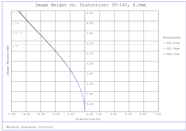
#35-141, 6mm, f/2.8 Cr Series Fixed Focal Length Lens, Distortion Plot
