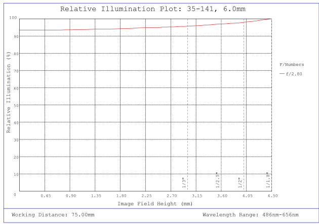
#35-141, 6mm, f/2.8 Cr Series Fixed Focal Length Lens, Relative Illumination Plot
