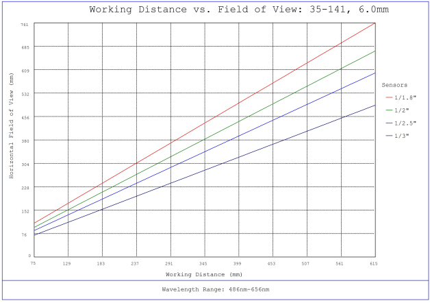
#35-141, 6mm, f/2.8 Cr Series Fixed Focal Length Lens, Working Distance versus Field of View Plot
