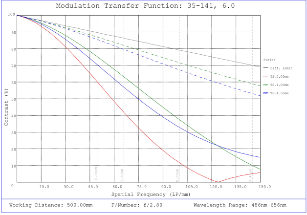
#35-141, 6mm, f/2.8 Cr Series Fixed Focal Length Lens, Modulated Transfer Function (MTF) Plot, 500mm Working Distance, f2.8
