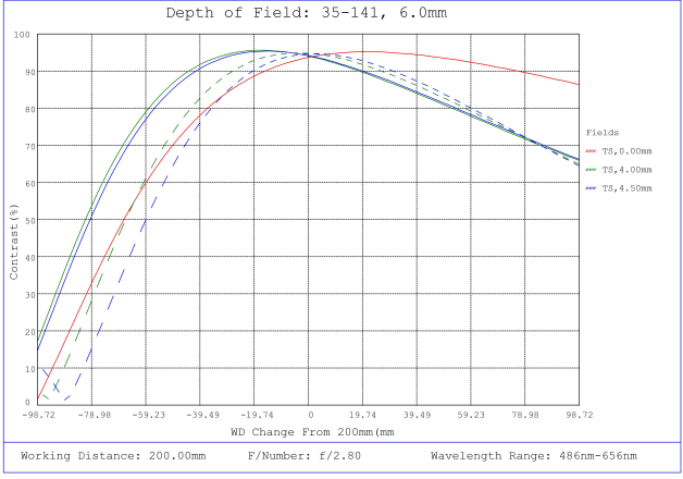
#35-141, 6mm, f/2.8 Cr Series Fixed Focal Length Lens, Depth of Field Plot, 200mm Working Distance, f2.8
