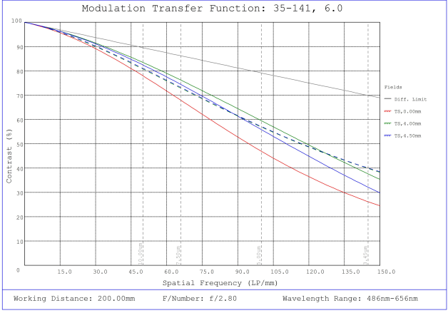
#35-141, 6mm, f/2.8 Cr Series Fixed Focal Length Lens, Modulated Transfer Function (MTF) Plot, 200mm Working Distance, f2.8
