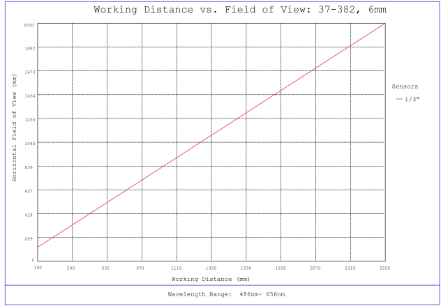
#37-382, 6mm FL f/2.5, Rugged Blue Series M12 Lens, Working Distance versus Field of View Plot
