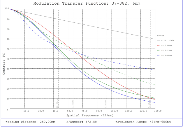
#37-382, 6mm FL f/2.5, Rugged Blue Series M12 Lens, Modulated Transfer Function (MTF) Plot, 250mm Working Distance, f2.5
