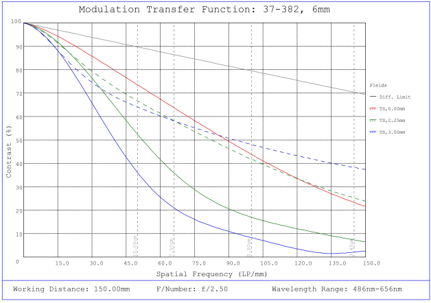
#37-382, 6mm FL f/2.5, Rugged Blue Series M12 Lens, Modulated Transfer Function (MTF) Plot, 150mm Working Distance, f2.5
