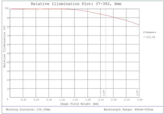
#37-382, 6mm FL f/2.5, Rugged Blue Series M12 Lens, Relative Illumination Plot
