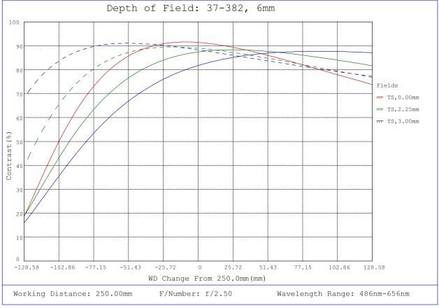
#37-382, 6mm FL f/2.5, Rugged Blue Series M12 Lens, Depth of Field Plot, 250mm Working Distance, f2.5
