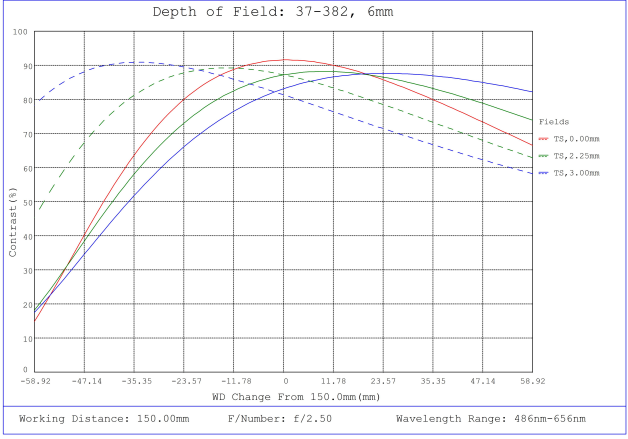
#37-382, 6mm FL f/2.5, Rugged Blue Series M12 Lens, Depth of Field Plot, 150mm Working Distance, f2.5
