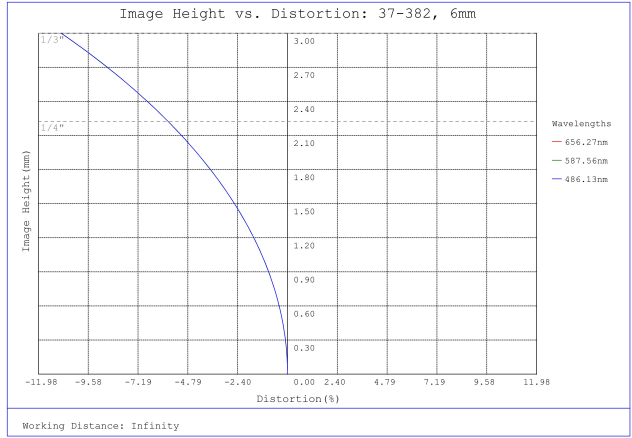
#37-382, 6mm FL f/2.5, Rugged Blue Series M12 Lens, Distortion Plot
