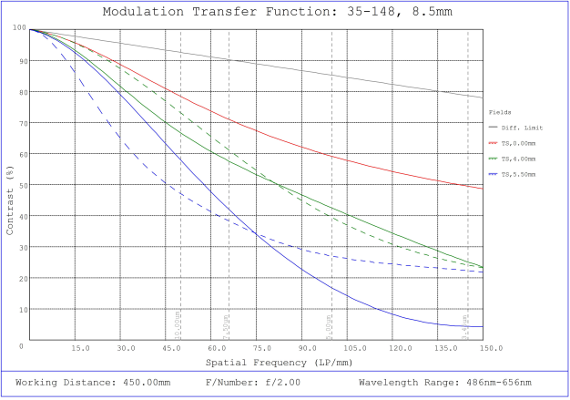
#35-148, 8.5mm, f/2.0, 75mm-∞ Primary WD, HRr Series Fixed Focal Length Lens, Modulated Transfer Function (MTF) Plot, 450mm Working Distance, f2
