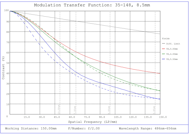
#35-148, 8.5mm, f/2.0, 75mm-∞ Primary WD, HRr Series Fixed Focal Length Lens, Modulated Transfer Function (MTF) Plot, 150mm Working Distance, f2
