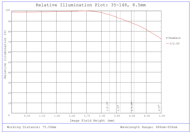
#35-148, 8.5mm, f/2.0, 75mm-∞ Primary WD, HRr Series Fixed Focal Length Lens, Relative Illumination Plot
