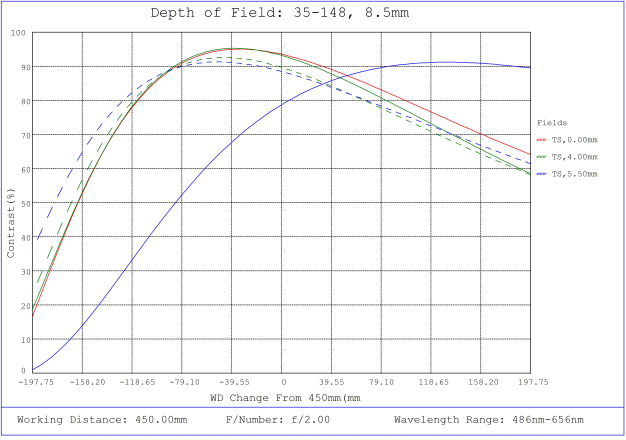
#35-148, 8.5mm, f/2.0, 75mm-∞ Primary WD, HRr Series Fixed Focal Length Lens, Depth of Field Plot, 450mm Working Distance, f2
