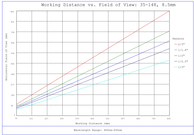
#35-148, 8.5mm, f/2.0, 75mm-∞ Primary WD, HRr Series Fixed Focal Length Lens, Working Distance versus Field of View Plot
