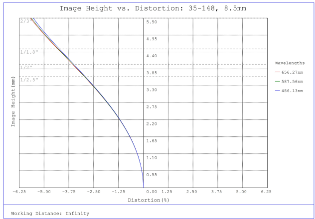
#35-148, 8.5mm, f/2.0, 75mm-∞ Primary WD, HRr Series Fixed Focal Length Lens, Distortion Plot
