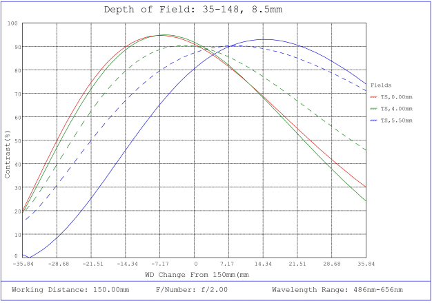
#35-148, 8.5mm, f/2.0, 75mm-∞ Primary WD, HRr Series Fixed Focal Length Lens, Depth of Field Plot, 150mm Working Distance, f2
