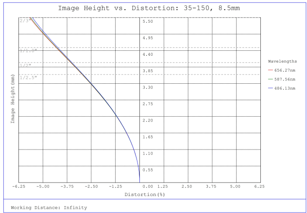
#35-150, 8.5mm, f/4.0, 75mm-∞ Primary WD, HRr Series Fixed Focal Length Lens, Distortion Plot
