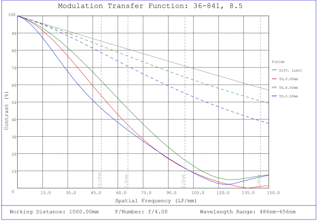
#36-841, 8.5mm, f/4 Cr Series Fixed Focal Length Lens, Modulated Transfer Function (MTF) Plot, 1000mm Working Distance, f4
