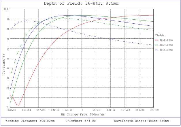
#36-841, 8.5mm, f/4 Cr Series Fixed Focal Length Lens, Depth of Field Plot, 500mm Working Distance, f4
