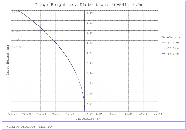
#36-841, 8.5mm, f/4 Cr Series Fixed Focal Length Lens, Distortion Plot
