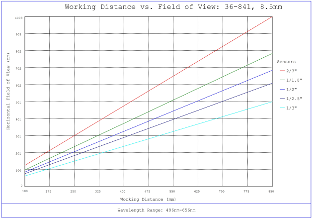
#36-841, 8.5mm, f/4 Cr Series Fixed Focal Length Lens, Working Distance versus Field of View Plot
