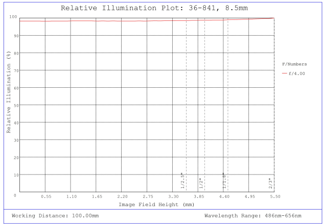
#36-841, 8.5mm, f/4 Cr Series Fixed Focal Length Lens, Relative Illumination Plot
