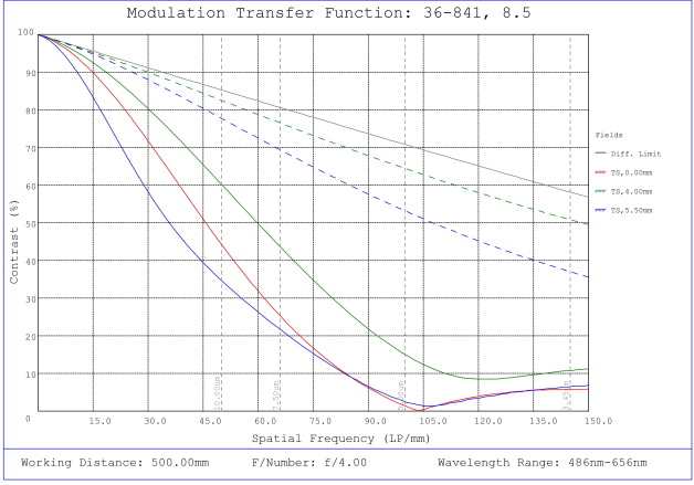
#36-841, 8.5mm, f/4 Cr Series Fixed Focal Length Lens, Modulated Transfer Function (MTF) Plot, 500mm Working Distance, f4
