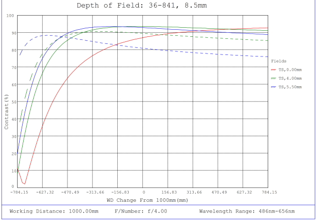
#36-841, 8.5mm, f/4 Cr Series Fixed Focal Length Lens, Depth of Field Plot, 1000mm Working Distance, f4
