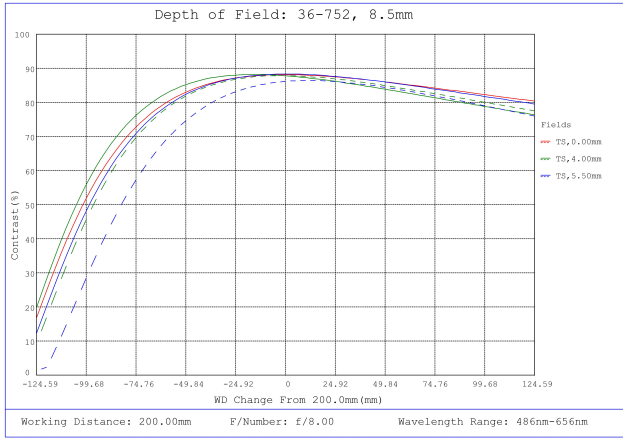
#36-752, 8.5mm f/8, 75mm-∞ Primary WD, HRi Series Fixed Focal Length Lens, Depth of Field Plot, 200mm Working Distance, f8
