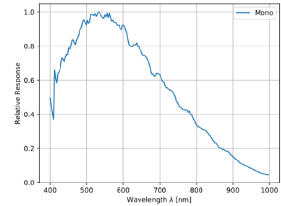
GMAX2505 Sensor QE Curve
