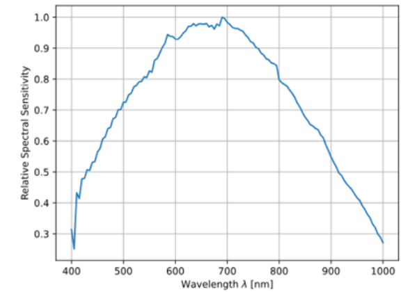
IMX900 Sensor QE Curve
