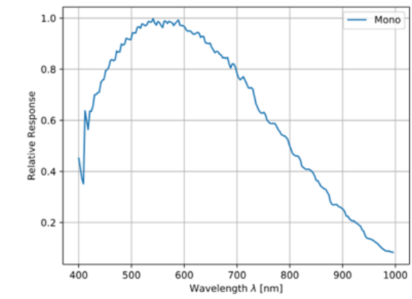
E2525A Sensor QE Curve
