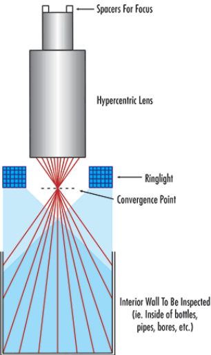
Hypercentric Lens Borescope Configuration
