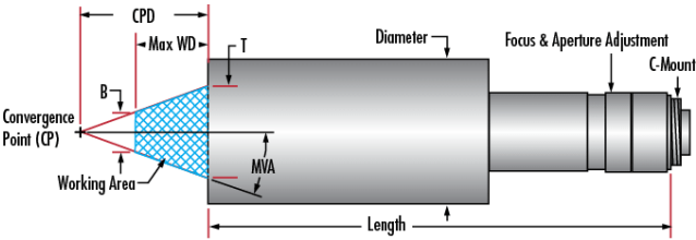
Hypercentric Lens External Viewing Configuration
