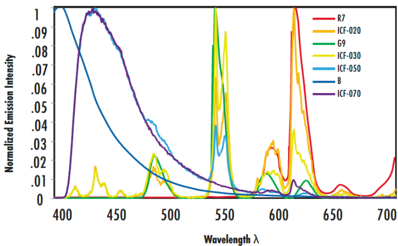
Fluorescent Glass Filters Emission 365nm Excitation
