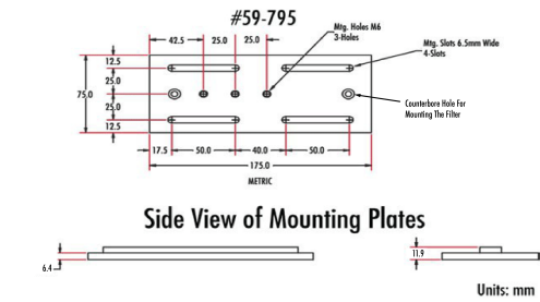
Top View of Mounting Plates
