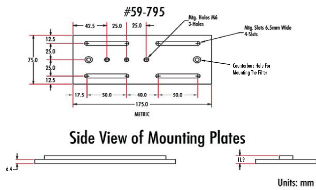
Top View of Mounting Plates
