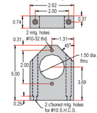
2.62" Z-Axis Adapter Plate (#54-379)
